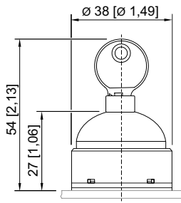
Key switch
