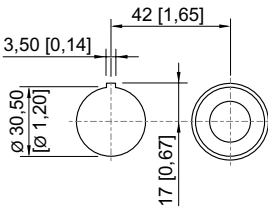
Drilling pattern: for aligning several devices \varnothing 38 mm, in a panel
