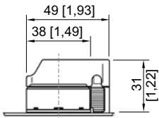
Control switch, one-time padlockable
